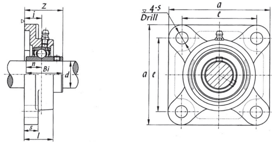
UCF 300 (heavy-duty)
