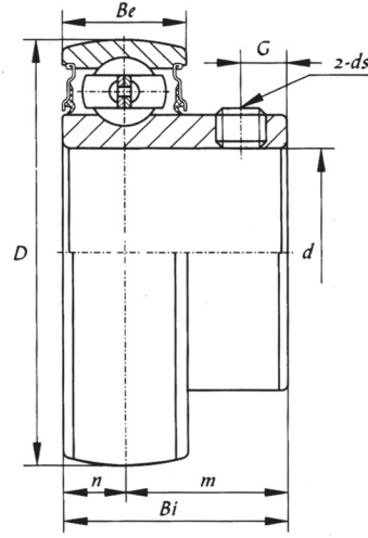
SB 200 (light-duty) Spherical O.D.
