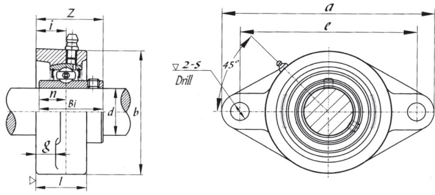
UCFL 200 (normal-duty)
