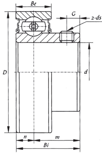
CSB 200 (light-duty) Cylindrical O.D.
