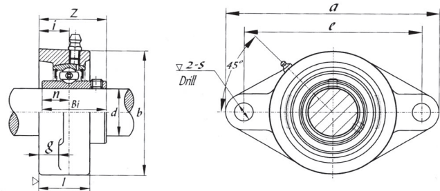
UCFL 300 (heavy-duty)
