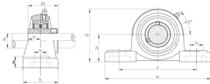
UCP 300 (heavy-duty)
